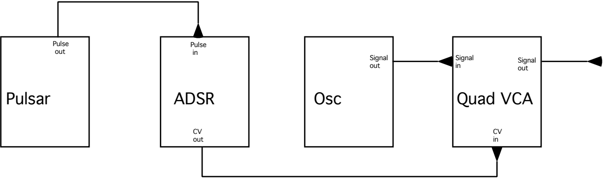
Typical Patch for controlling volume of an oscillator
